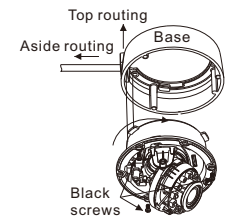
Figure 3-6 Installing base
