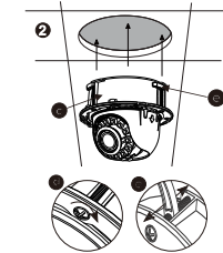
Figure 3-9 Embedded Installation
