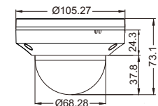
Figure 2-4 Dimensions (Unit:mm)
