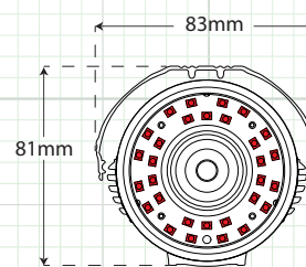
Camera Dimensions
