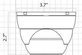
Camera Dimensions
