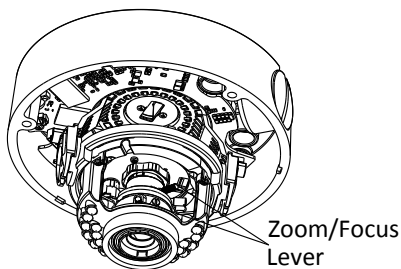
Figure 2-15 Lens Adjustment
