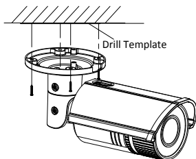
Figure 2-6 Secure the Camera
