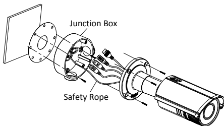
Figure 2-8 Mounting with a Junction Box
