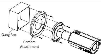
Figure 2-9 Mounting with a Gang Box
