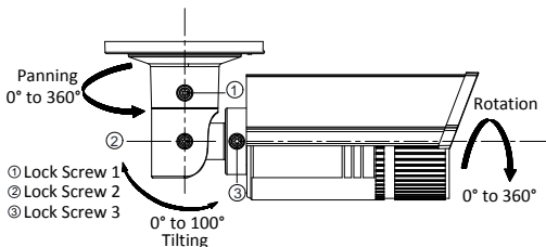
Figure 2-7 View Angle Adjustment
