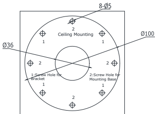
Figure 2-5 Drilling Holes in the Wall
