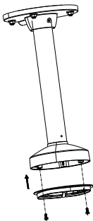
Figure 2-11 Fix the Adapter Plate
