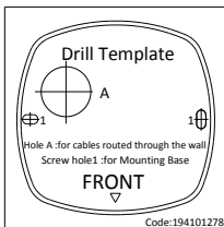
Figure 2-1 Drill Template
