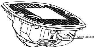
Figure 2-19 Install and Uninstall Micro SD Card
