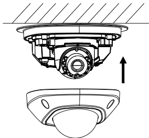
Figure 2-5 Install the Front Cover
