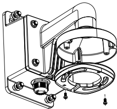
Figure 2-15 Fix the Adapter Plate
