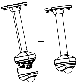
Figure 2-13 Install the Front Cover
