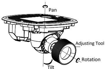
Figure 2-4 3-Axis Adjustment
