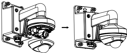
Figure 2-17 Install the Front Cover
