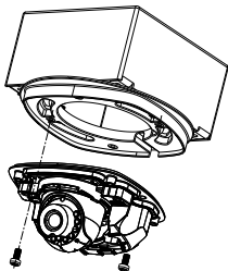
Figure 2-9 Fix the Dome Drive
