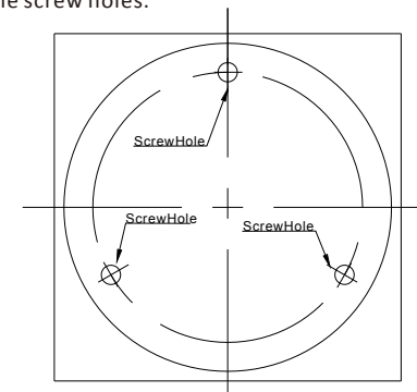
Figure 2-1 Drill Template
