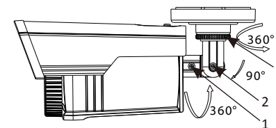
Figure 2-3 3-axis Adjustment
