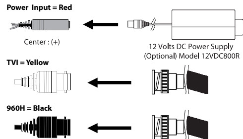
In-Line Cable Mounted OSD Control
