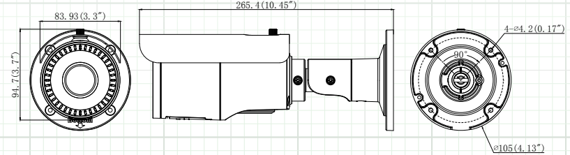
Camera Overview
